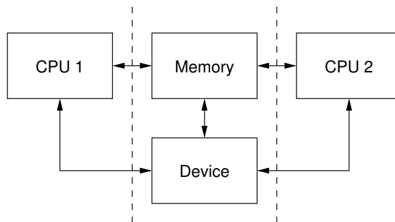
Figure 14.8: Abstract Memory Access Model
