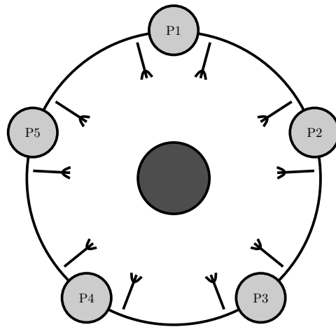
Figure C.3: Dining Philosophers Problem, Fully Partitioned
