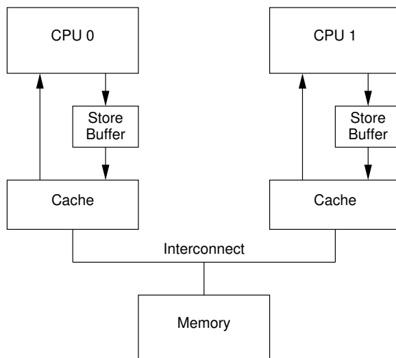
Figure B.5: Caches With Store Buffers
