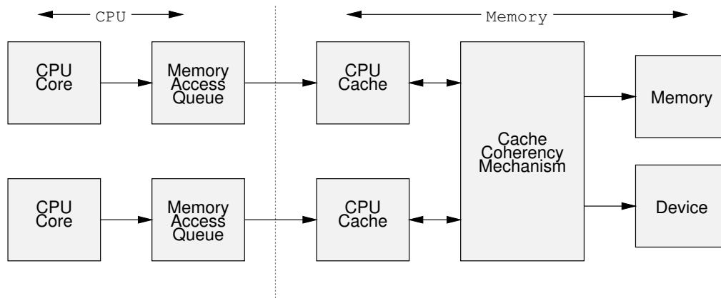
Figure 14.19: Memory Architecture
