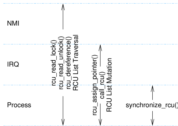
Figure 9.46: RCU API Usage Constraints
