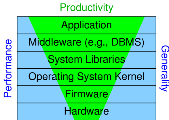
Figure 2.3: Software Layers and Performance, Productivity, and Generality
