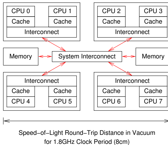
Figure 7.13: System Architecture and Lock Unfairness
