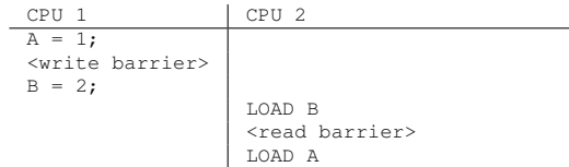
Figure 14.12: Read Barrier Needed
